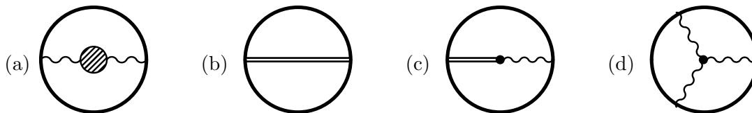
Figure 1: The two-loop Feynman diagrams contributing to a circular \langle W \rangle . The bold circular line represents the Wilson loop contour, whereas wiggly lines denote gluon and straight lines scalar propagators.
